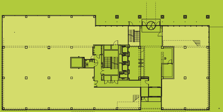
Rzut parteru Ground floor plan
