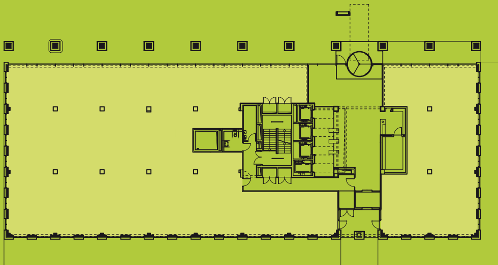
Rzut parteru Ground floor plan
